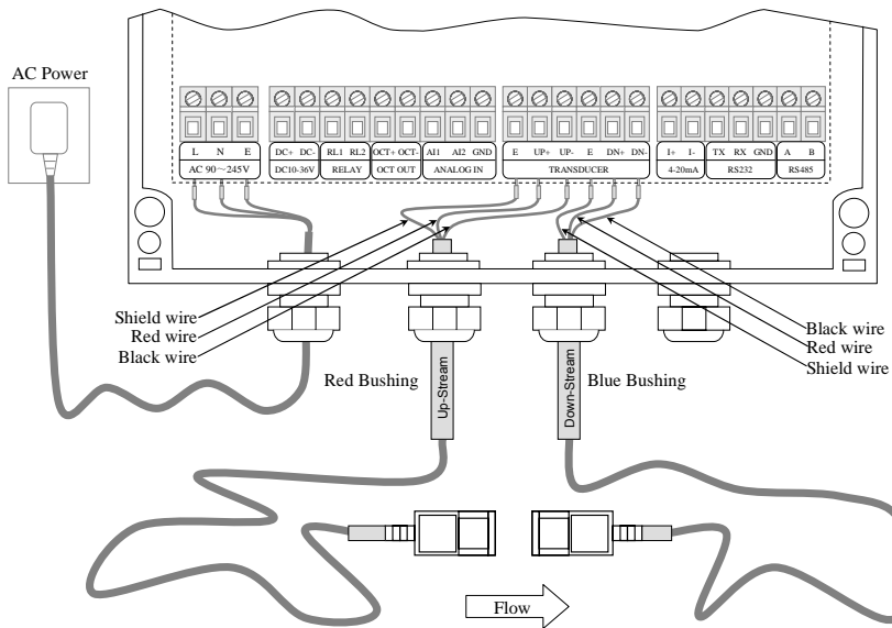
Figure ( 2-1) Connection of the flow meter's transducers
